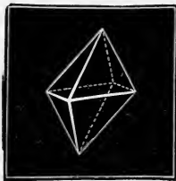
Crystal of Washing-Soda.
